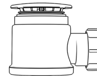
Product Code: WTSH40 Description: 1 1/2" Shower Trap (50mm Tray) Seal: 50mm
